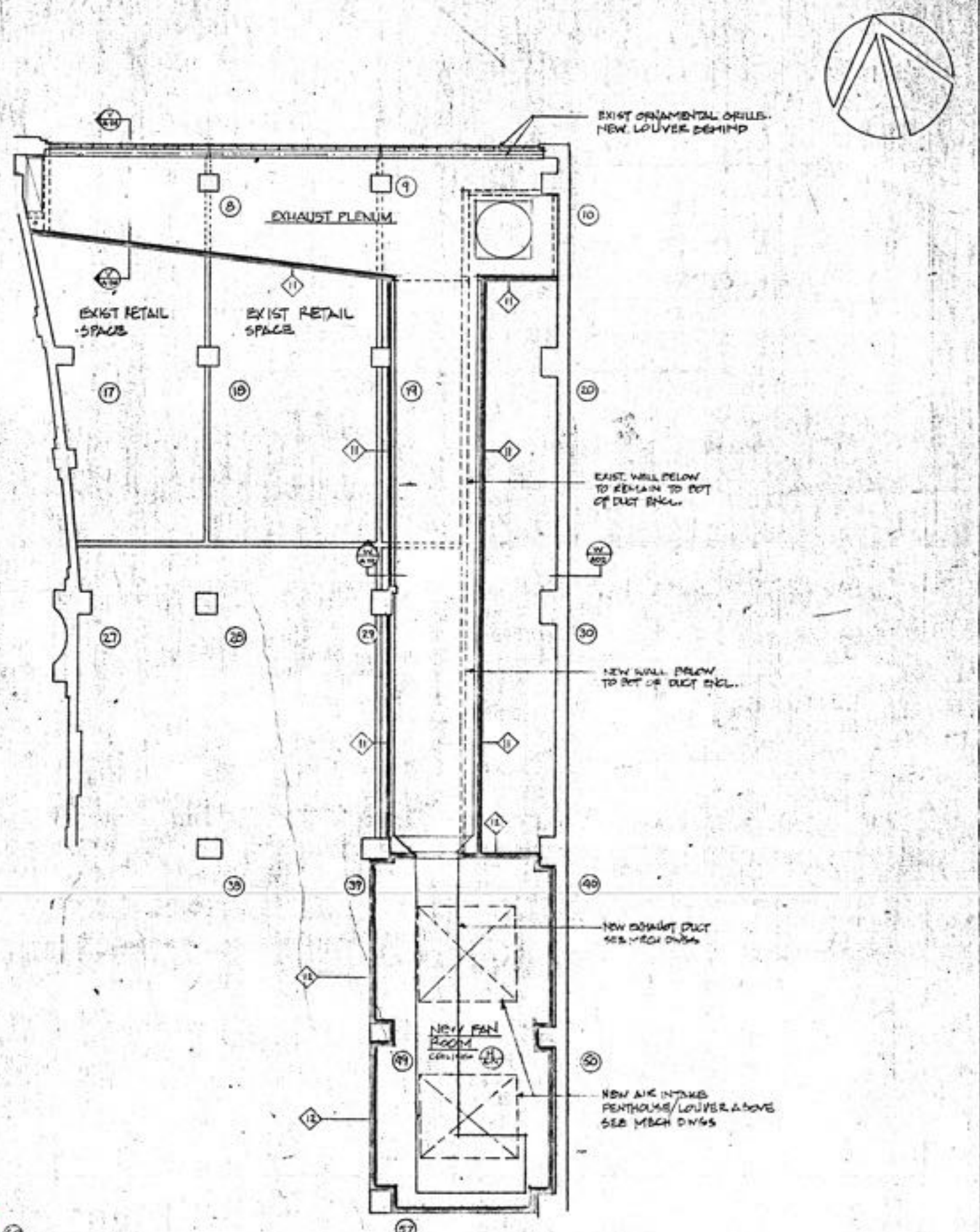
1 ST FLOOR: EXHAUST DUCT
